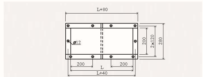
Manually-operated cascade magnet system without valve box.
